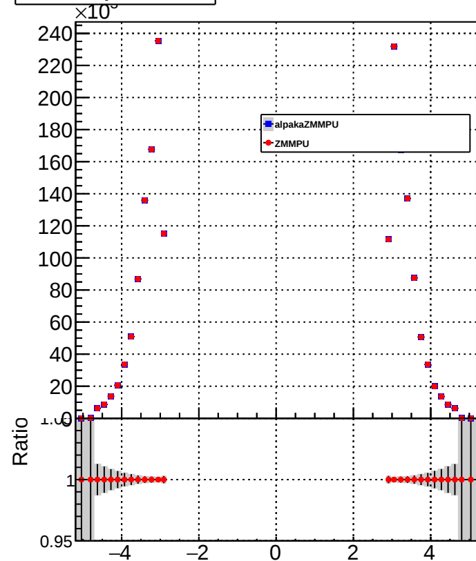
HF_EM_particleEta
