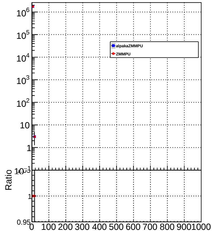
HF_EM_particlePtHigh
