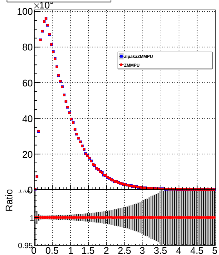
HF_EM_particlePtLow
