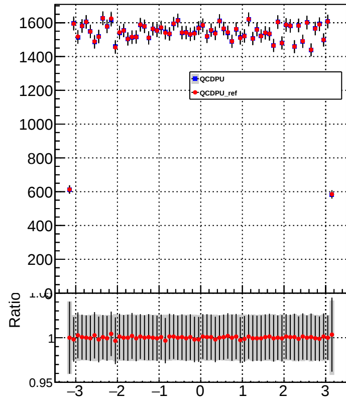
CorrJetPhi Pt>20
