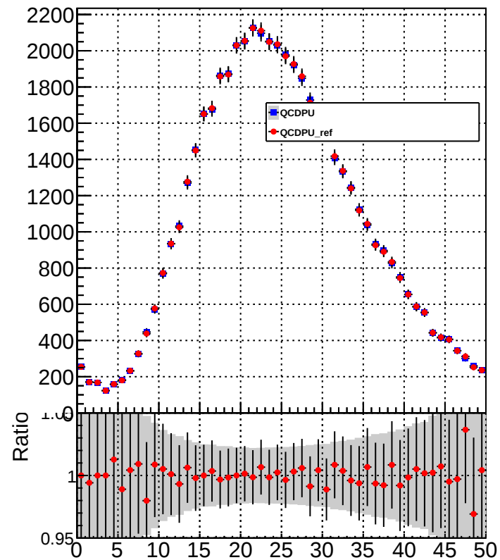
chargedHadronMultiplicity
