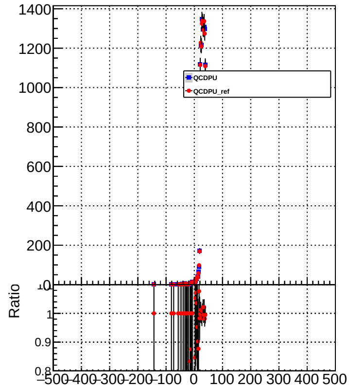
METResolution_GenMETTrue_MET20to40
