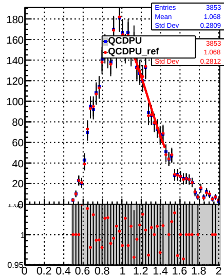
Jet response ( p_T/p_{Tgen} ) in 15 \leq p_T < 21 , 0.0 \leq |\eta| < 1.3
