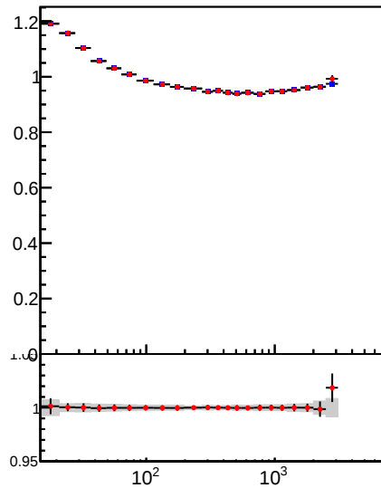
Raw Jet pT response, 0.5 < |\eta| < 1.3
