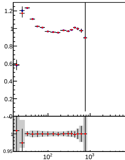
Raw Jet pT response, 2.5 < |\eta| < 3.0
