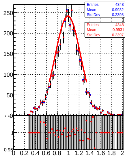
Jet response (pT/pTgen) in 28 \leq p_t < 37 , 0.5 \leq |\eta| < 2.1
