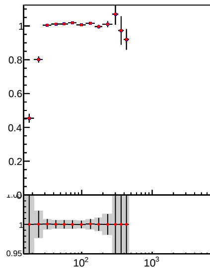
Jet pT response, 3.0 < |\eta| < 5.0
