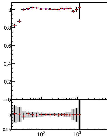
Jet pT response, 2.1 < |\eta| < 2.5
