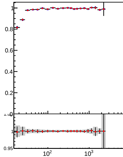
Jet pT response, 1.3 < |\eta| < 2.1
