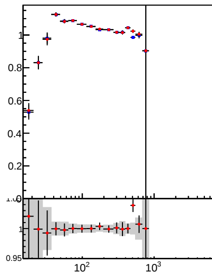
Jet pT response, 2.5 < |\eta| < 3.0
