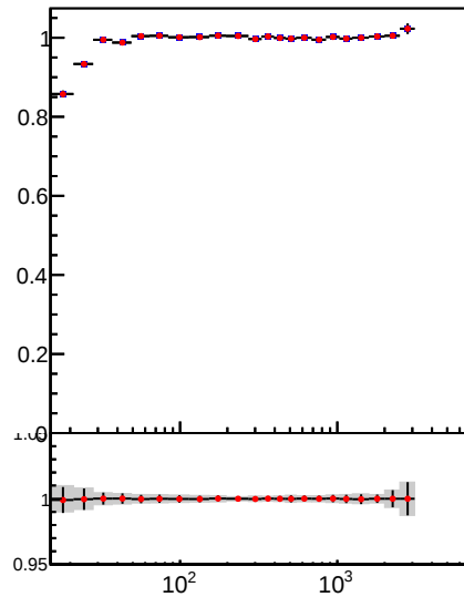
Jet pT response, 0.5 < |\eta| < 1.3
