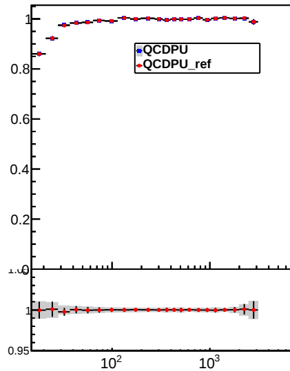
Jet pT response, 0.0 < |\eta| < 0.5
