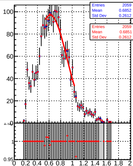
Raw Jet response (pT/pTgen) in 28 &lt;= pt &lt; 37, 3.0 &lt;= |eta| &lt; 5.0
