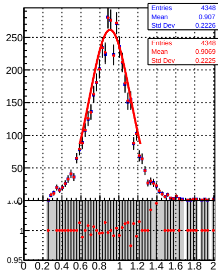
Raw Jet response (pT/pTgen) in 28 &lt;= pt &lt; 37, 0.5 &lt;= |eta| &lt; 1.3
