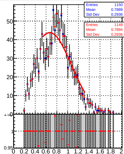
Raw Jet response (pT/pTgen) in 28 &lt;= pt &lt; 37, 2.5 &lt;= |eta| &lt; 3.0
