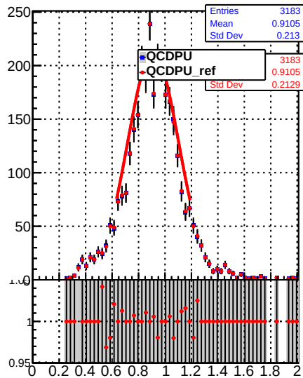
Raw Jet response (pT/pTgen) in 28 &lt;= pt &lt; 37, 0.0 &lt;= |eta| &lt; 0.5
