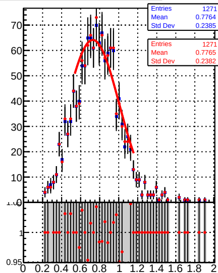
Raw Jet response (pT/pTgen) in 28 &lt;= pt &lt; 37, 2.1 &lt;= |eta| &lt; 2.5
