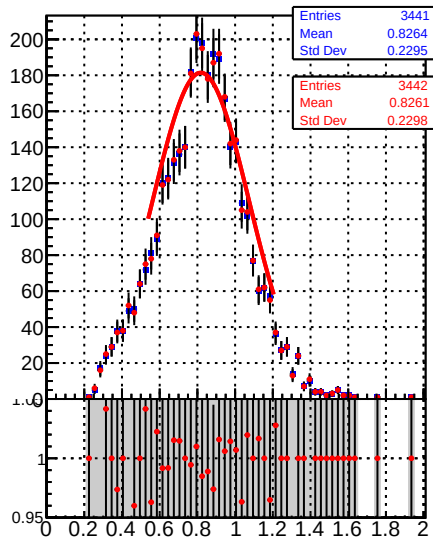
Raw Jet response (pT/pTgen) in 28 &lt;= pt &lt; 37, 1.3 &lt;= |eta| &lt; 2.1
