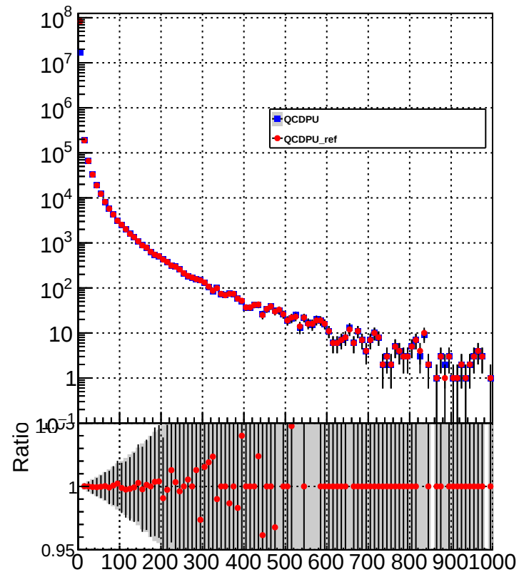
chargedHadronPtHigh
