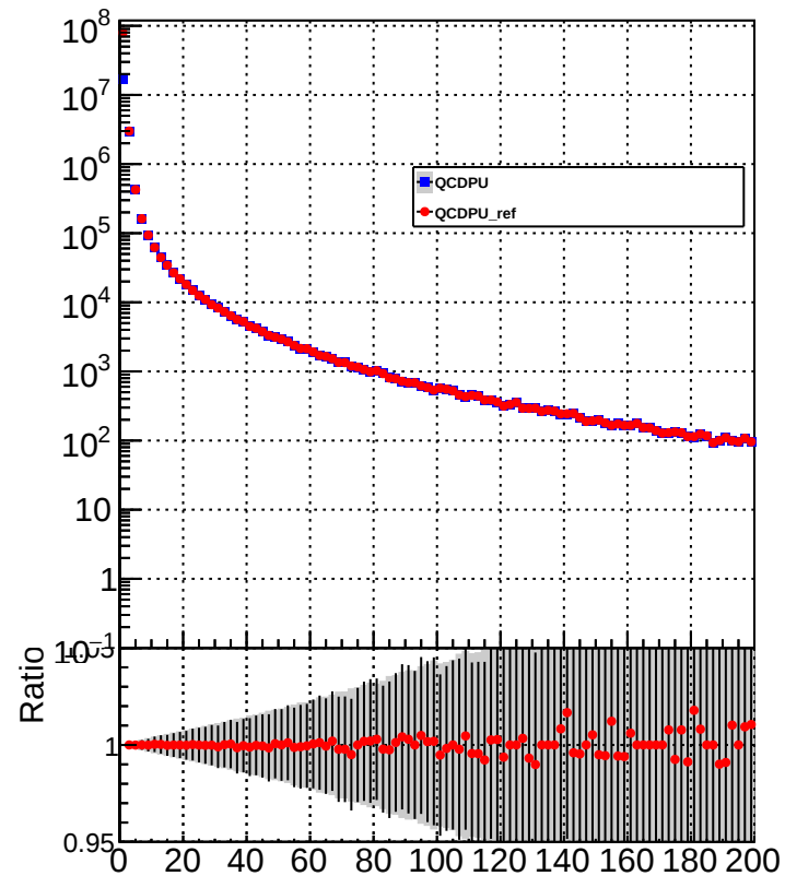
chargedHadronPtMid
