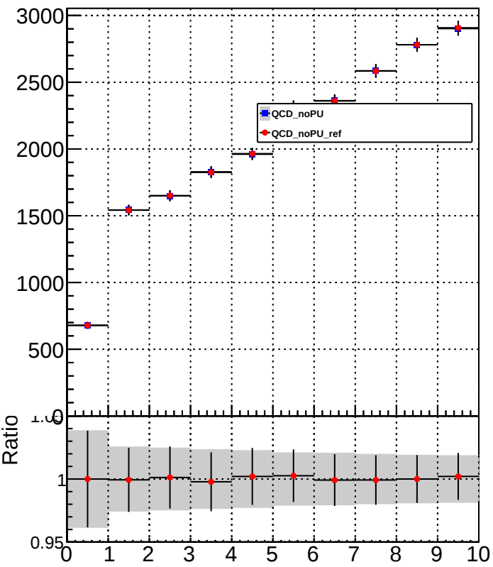
photonMultiplicity
