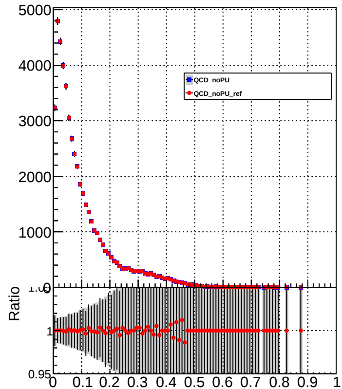
HFHadronEtFraction
