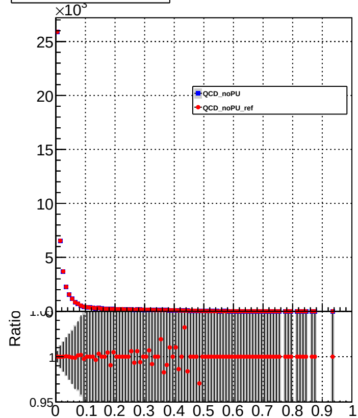
HFHadronEtFraction
