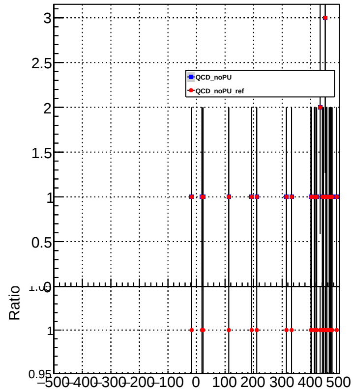
METResolution_GenMETTrue_MET400to500
