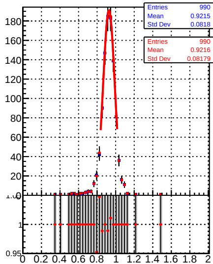
Raw Jet response (pT/pTgen) in 548 &lt;= pt &lt; 686, 1.3 &lt;= |eta| &lt; 2.1
