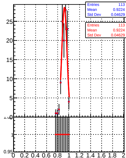
Raw Jet response (pT/pTgen) in 548 &lt;= pt &lt; 686, 2.1 &lt;= |eta| &lt; 2.5
