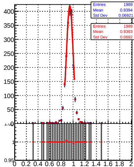
Raw Jet response (pT/pTgen) in 548 &lt;= pt &lt; 686, 0.5 &lt;= |eta| &lt; 1.3
