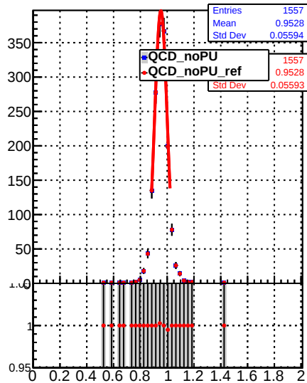
Raw Jet response (pT/pTgen) in 548 &lt;= pt &lt; 686, 0.0 &lt;= |eta| &lt; 0.5
