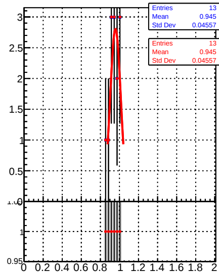
Raw Jet response (pT/pTgen) in 548 &lt;= pt &lt; 686, 2.5 &lt;= |eta| &lt; 3.0
