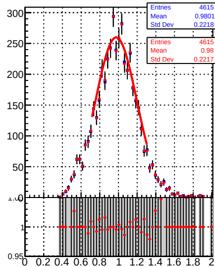
Jet response (pT/pTgen) in 21 <= pt < 28, 1.3 <= |eta| < 2.1
