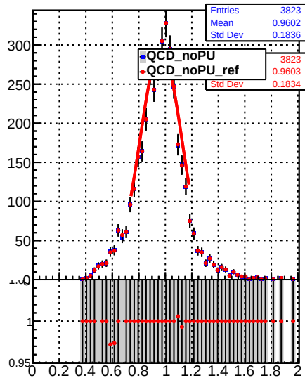
Jet response (pT/pTgen) in 21 <= pt < 28, 0.0 <= |eta| < 0.5
