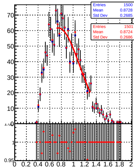
Jet response (pT/pTgen) in 21 <= pt < 28, 2.5 <= |eta| < 3.0
