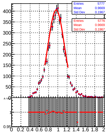
Jet response (pT/pTgen) in 21 <= pt < 28, 0.5 <= |eta| < 1.3
