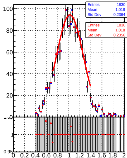
Jet response (pT/pTgen) in 21 <= pt < 28, 2.1 <= |eta| < 2.5
