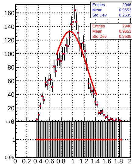
Jet response (pT/pTgen) in 21 <= pt < 28, 3.0 <= |eta| < 5.0
