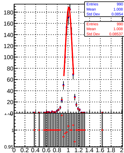
Jet response (pT/pTgen) in 548 \leq p_t < 686 , 1.3 \leq |\eta| < 2.1
