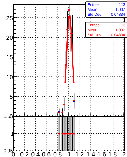
Jet response (pT/pTgen) in 548 \leq p_t < 686 , 2.1 \leq |\eta| < 2.5
