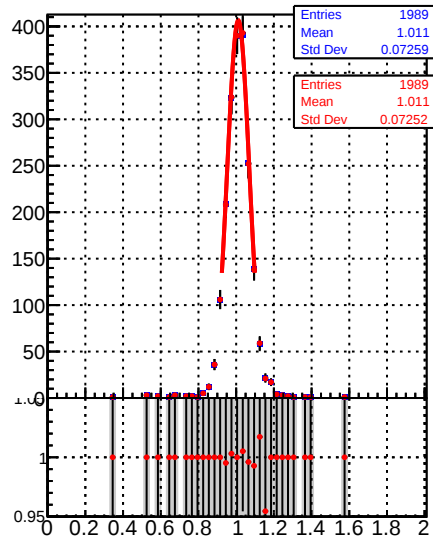
Jet response (pT/pTgen) in 548 \leq p_t < 686 , 0.5 \leq |\eta| < 1.3
