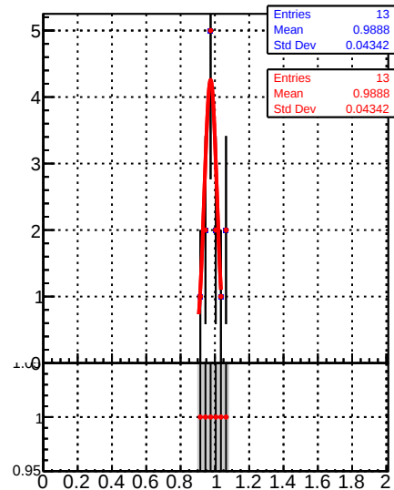
Jet response (pT/pTgen) in 548 \leq p_t < 686 , 2.5 \leq |\eta| < 3.0
