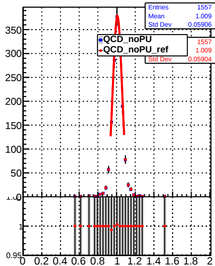
Jet response (pT/pTgen) in 548 \leq p_t < 686 , 0.0 \leq |\eta| < 0.5
