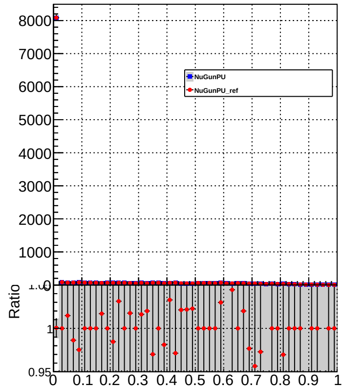
chargedHadronEnergyFraction
