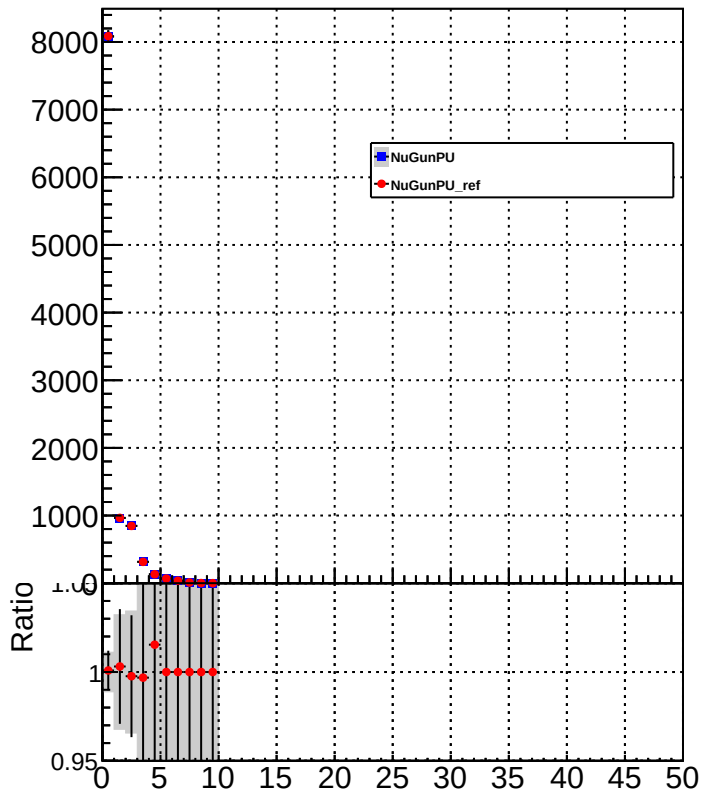
neutralHadronMultiplicity
