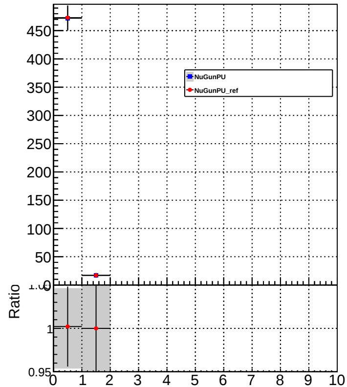
muonMultiplicity
