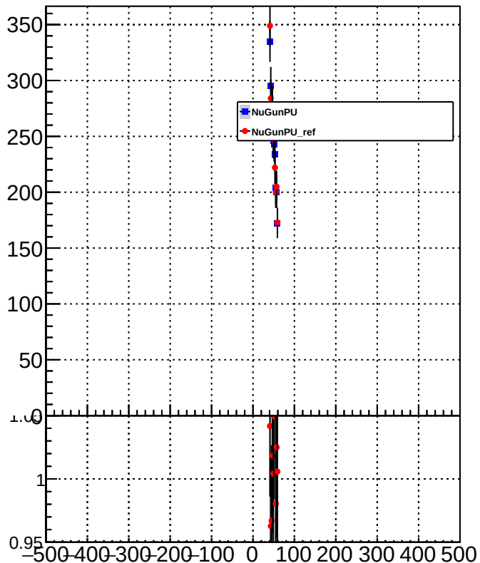
METResolution_GenMETTrue_MET40to60
