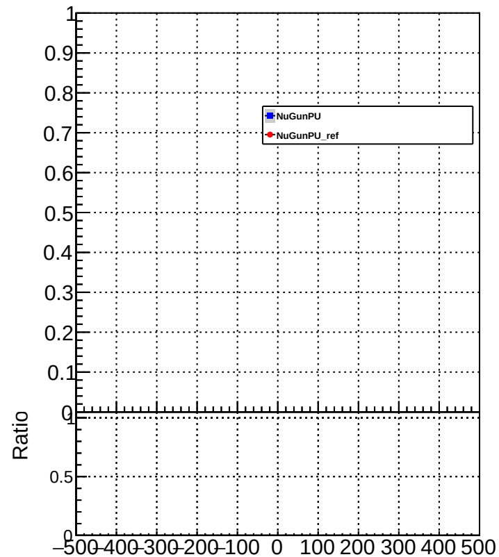
METResolution_GenMETTrue_MET150to200
