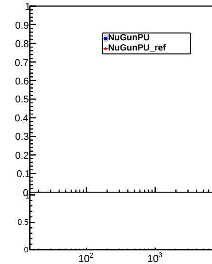
Jet pT resolution, 0.0 < |\eta| < 0.5
