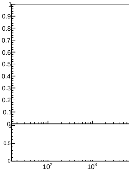
Raw Jet pT resolution using RMS, 2.1 < |\eta| < 2.5
