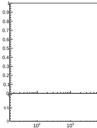
Raw Jet pT resolution using RMS, 3.0 < |\eta| < 5.0
