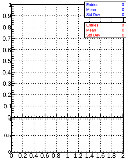
Raw Jet response (pT/pTgen) in 196 &lt;= pt &lt; 272, 2.1 &lt;= |eta| &lt; 2.5
