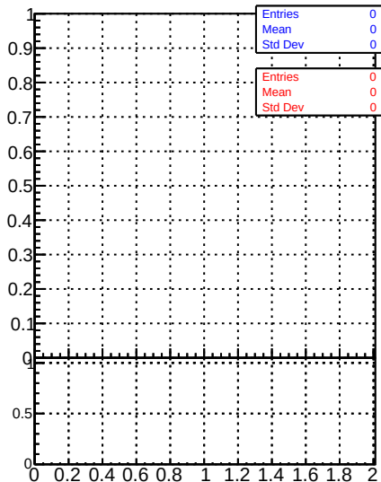
Raw Jet response (pT/pTgen) in 196 &lt;= pt &lt; 272, 2.5 &lt;= |eta| &lt; 3.0
