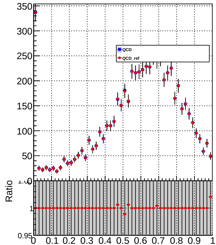
chargedHadronEnergyFraction
