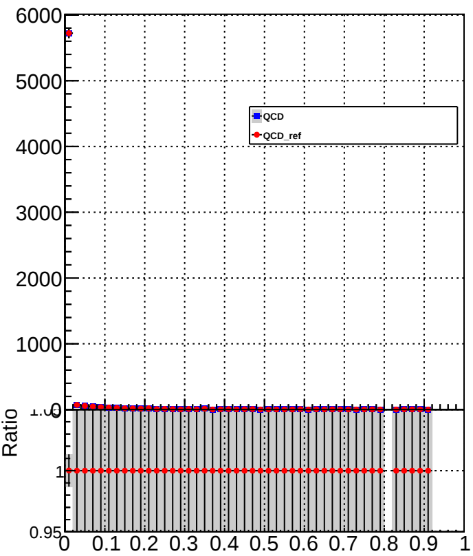
electronEnergyFraction
