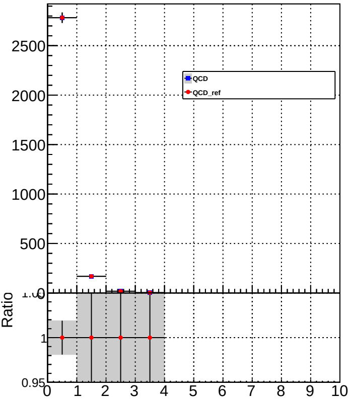
muonMultiplicity
