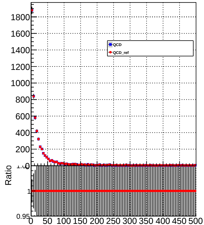
neutralHadronEnergy
