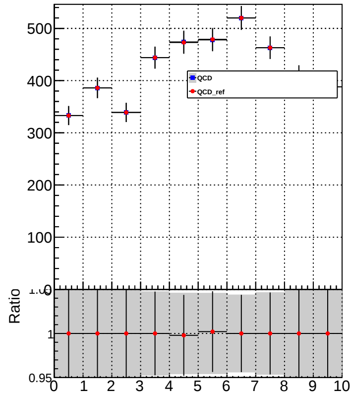
photonMultiplicity
