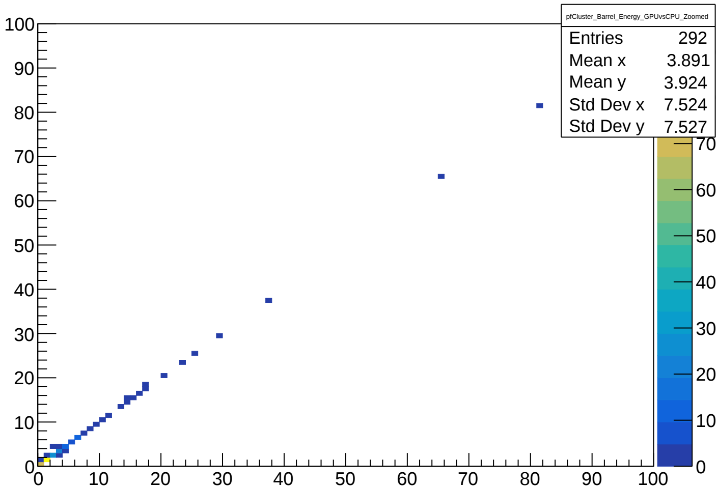
pfCluster_Barrel_Energy_GPUvsCPU_Zoomed
