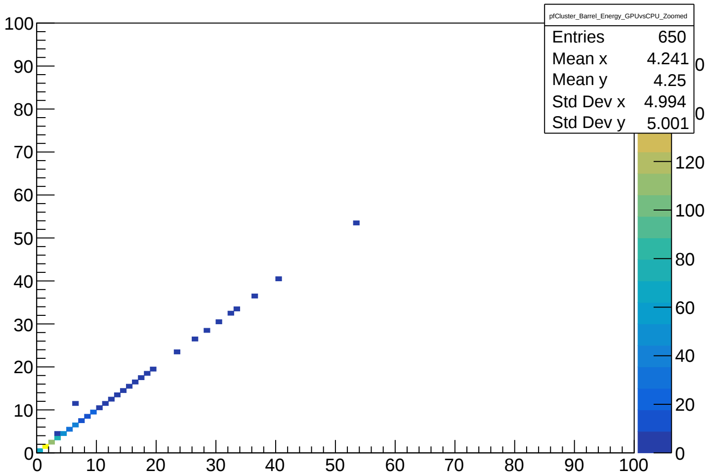
pfCluster_Barrel_Energy_GPUvsCPU_Zoomed
