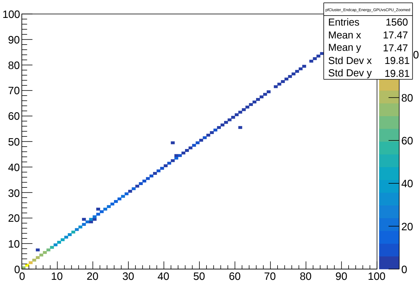
pfCluster_Endcap_Energy_GPUvsCPU_Zoomed
