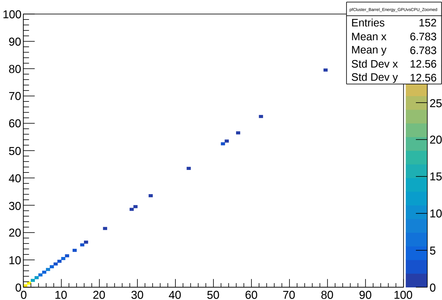
pfCluster_Barrel_Energy_GPUvsCPU_Zoomed
