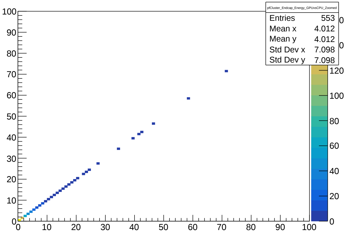
pfCluster_Endcap_Energy_GPUvsCPU_Zoomed
