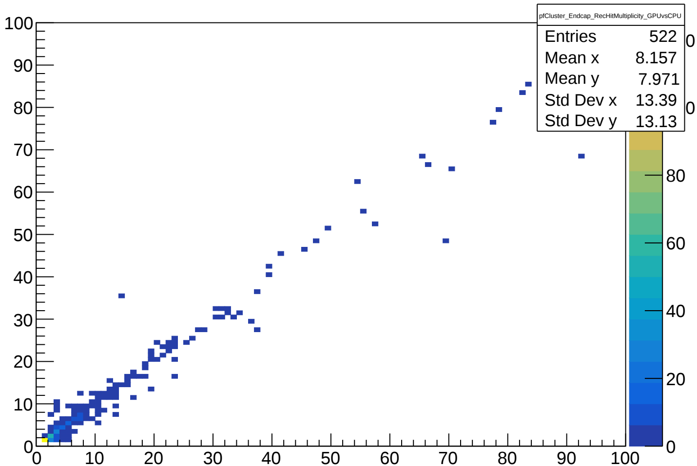
pfCluster_Endcap_RecHitMultiplicity_GPUvsCPU
