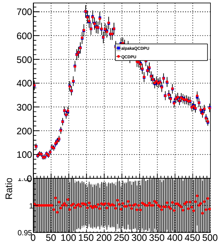
chargedHadronEnergy
