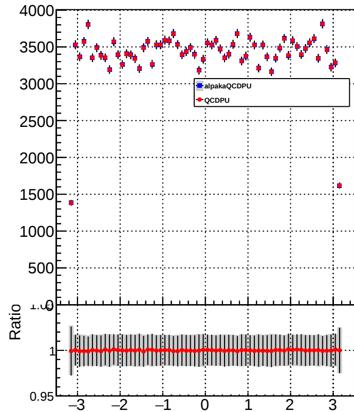
CorrJetPhi Pt>20
