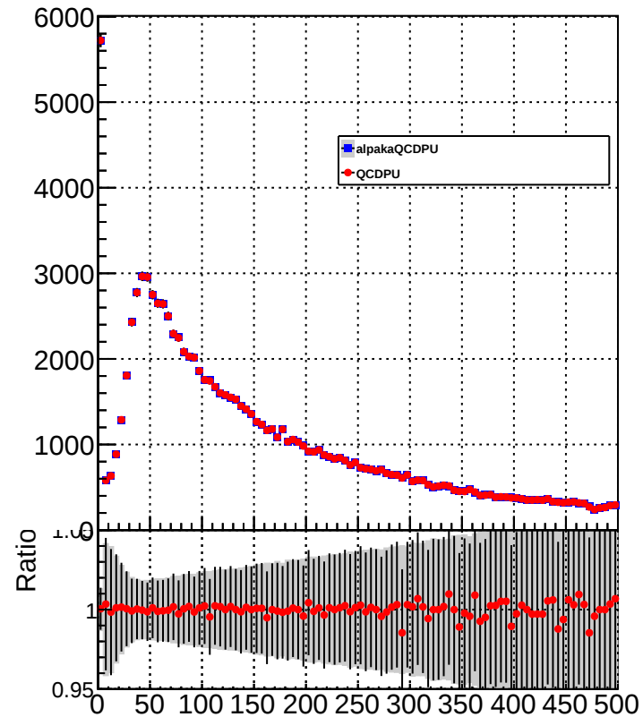
chargedHadronEnergy
