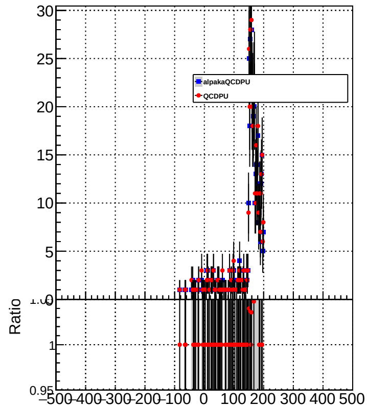
METResolution_GenMETTrue_MET150to200
