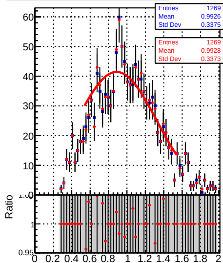
Jet response (pT/pTgen) in 28 \leq p_t < 37 , 2.5 \leq |\eta| < 3.0
