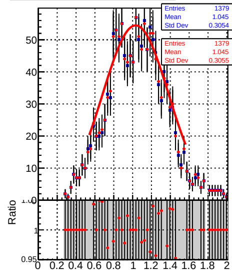
Jet response (pT/pTgen) in 28 \leq p_t < 37 , 2.1 \leq |\eta| < 2.5
