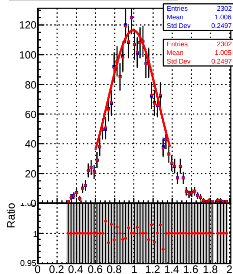
Jet response (pT/pTgen) in 28 \leq p_t < 37 , 3.0 \leq |\eta| < 5.0
