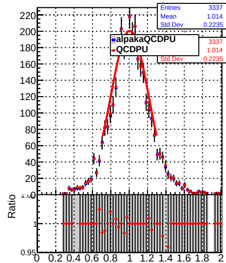
Jet response (pT/pTgen) in 28 \leq p_t < 37 , 0.0 \leq |\eta| < 0.5
