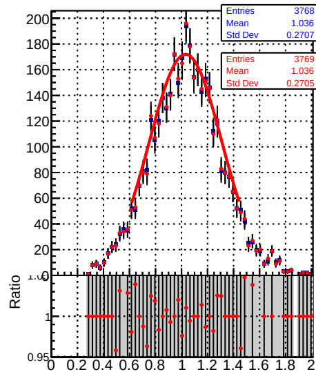
Jet response (pT/pTgen) in 28 \leq p_t < 37 , 1.3 \leq |\eta| < 2.1
