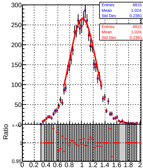
Jet response (pT/pTgen) in 28 \leq p_t < 37 , 0.5 \leq |\eta| < 1.3
