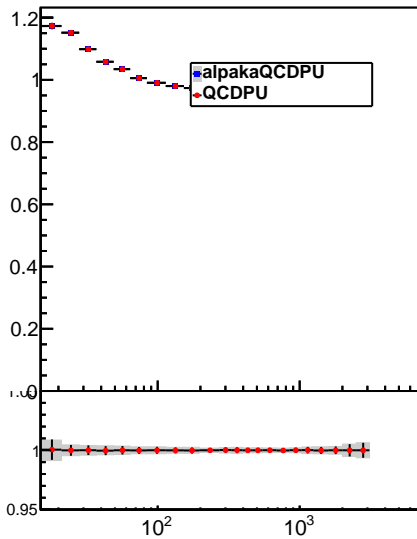
Raw Jet pT response, 0.0 < |\eta| < 0.5
