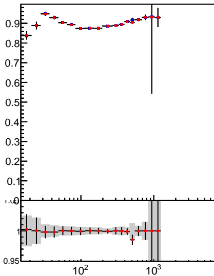
Raw Jet pT response, 2.1 < |\eta| < 2.5
