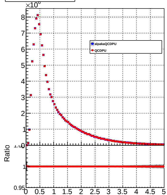
AllCandidatePtLow
