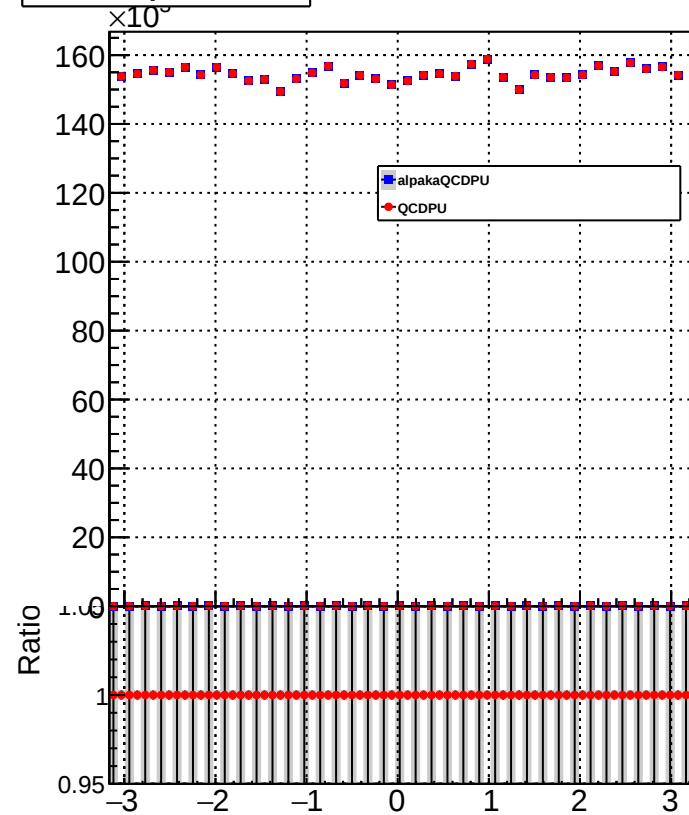
HF_EM_particlePhi
