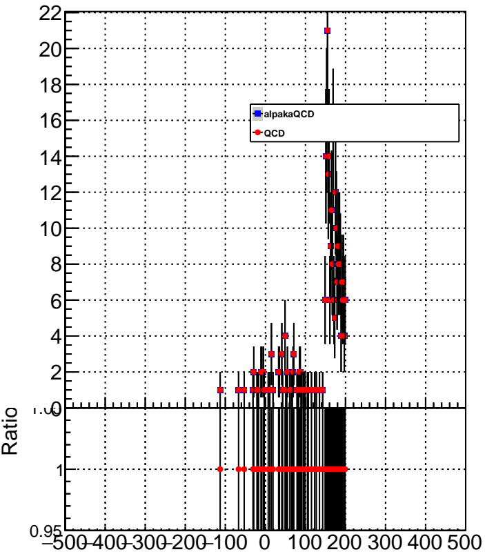
METResolution_GenMETTrue_MET150to200
