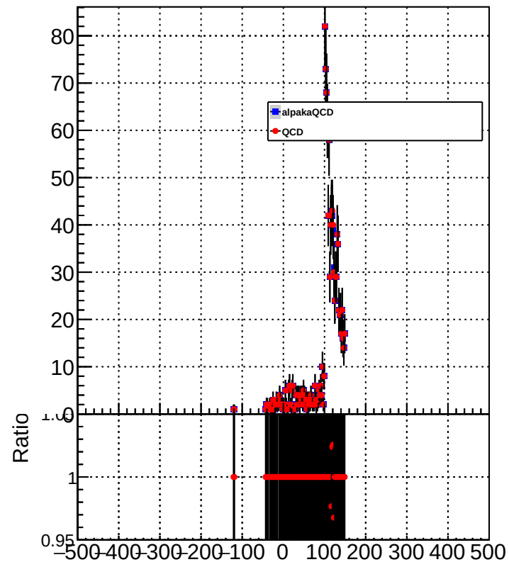
METResolution_GenMETTrue_MET100to150
