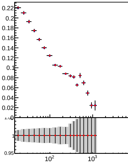
Jet pT resolution using RMS, 2.1 < |\eta| < 2.5
