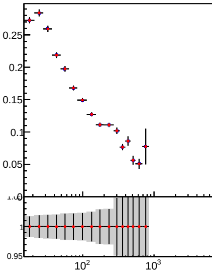
Jet pT resolution using RMS, 2.5 < |\eta| < 3.0
