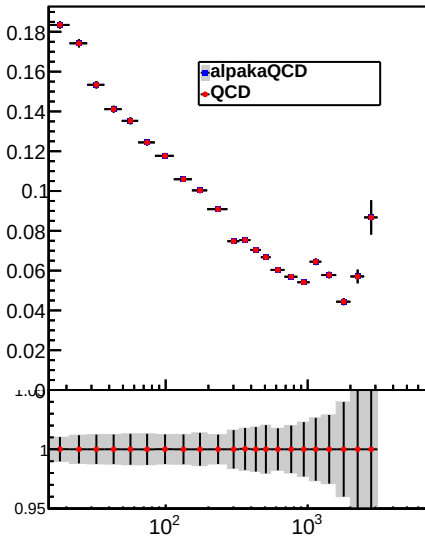
Jet pT resolution using RMS, 0.0 < |\eta| < 0.5
