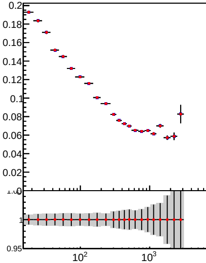
Jet pT resolution using RMS, 0.5 < |\eta| < 1.3
