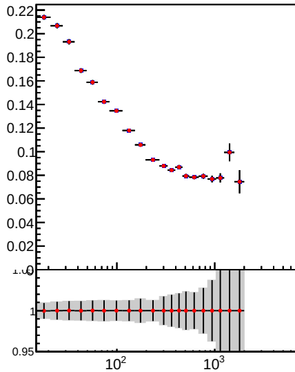
Jet pT resolution using RMS, 1.3 < |\eta| < 2.1
