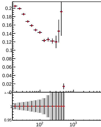
Jet pT resolution using RMS, 3.0 < |\eta| < 5.0
